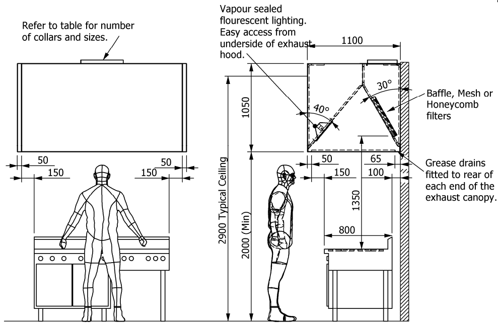
Hood Data – Hood mounted against the wall.
