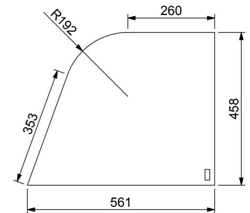
Glass End Dimensions
