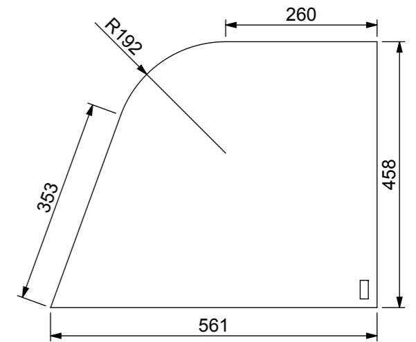
Glass End Dimensions
