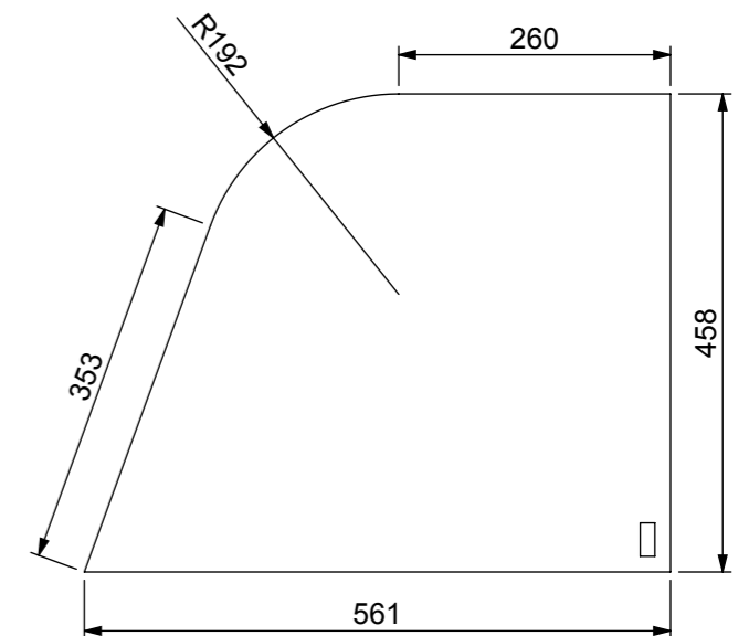
Glass End Dimensions
